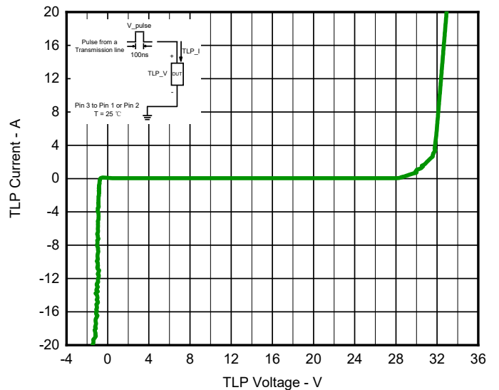
Fig 6. TLP Measurement
