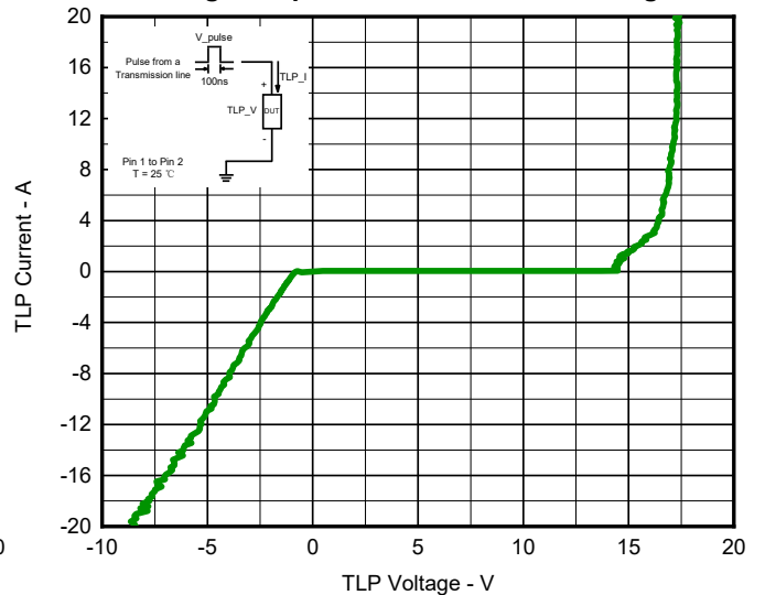
Fig 6. TLP Measurement
