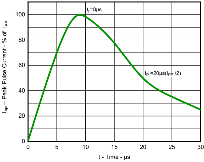
Fig 1. Pulse Waveform(8/20µs)
