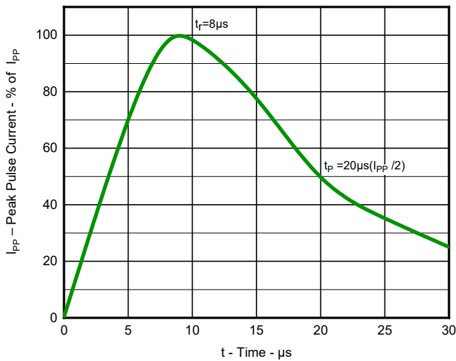
Fig 1. Pulse Waveform
