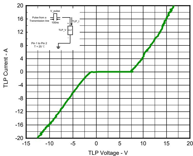
Fig 5. TLP Measurement
