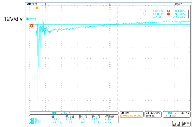
Fig 8. ESD clamping voltage (IEC61000-4-2 -8KV contact)
