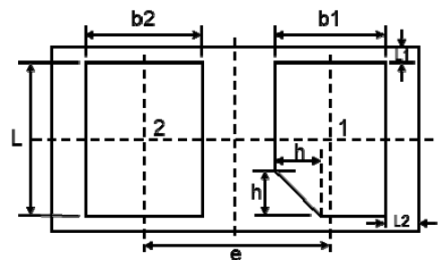
Bottom View (Optional)
