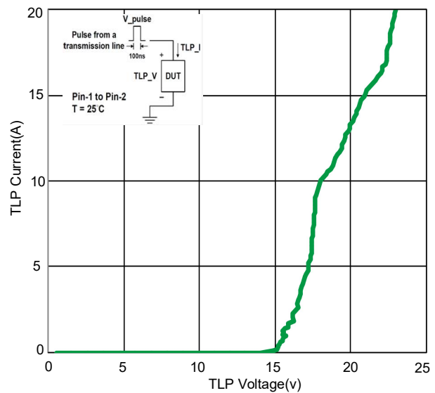
Fig 6. TLP Measurement
