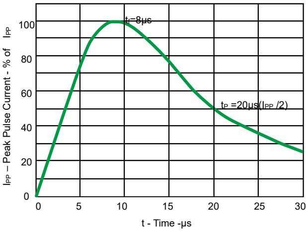
Fig 1. Pulse Waveform
