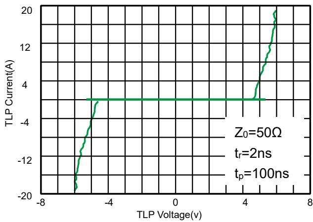
Fig 3. TLP Measurement
