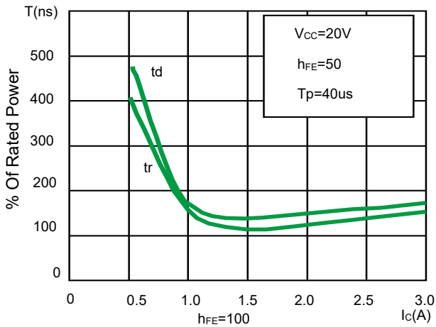
Fig 5. Switching Times Resistive Load
