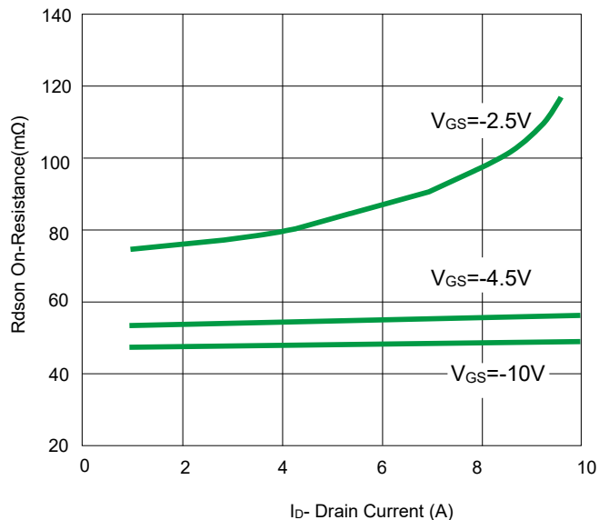
Fig 4. Drain-Source On-Resistance
