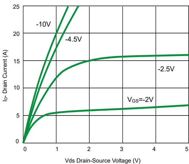
Fig 3. Output Characteristics
