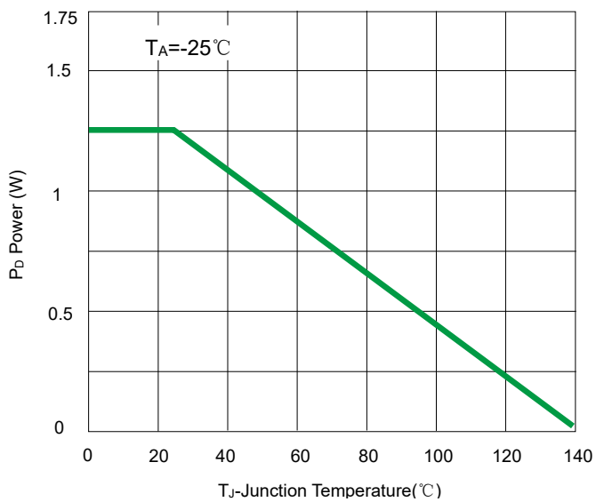
Fig 1. Power Dissipation
