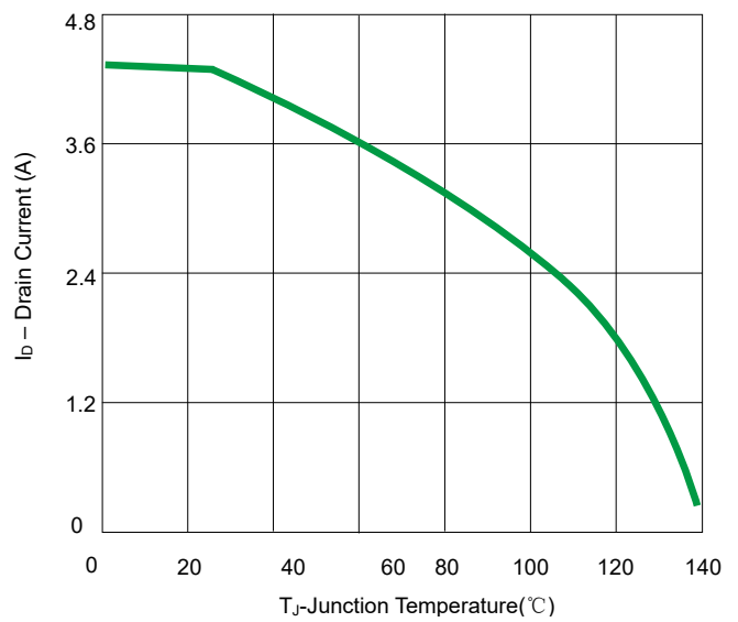
Fig 2. Drain Current
